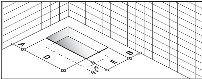
A = 760 mm / 29 15/16" - B = 400 mm / 15 3/4" - C = 120 mm / 4 3/4" - D = 400 mm / 15 3/4" - E = 150 mm / 5 15/16"
