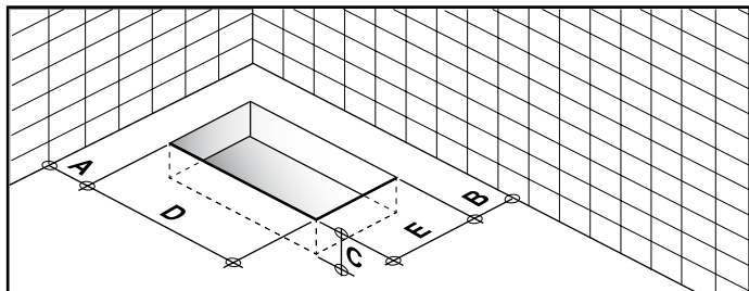
A = 850 mm / 33 7/16" - B = 425 mm / 16 3/4" - C = 70 mm / 2 3/4" - D = 400 mm / 15 3/4" - E = 150 mm / 5 15/16"
