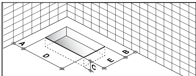
A = 670 mm / 26 3/8" - B = 370 mm / 14 9/16" - C = 120 mm / 4 3/4" - D = 400 mm / 15 3/4" - E = 150 mm / 5 15/16"
