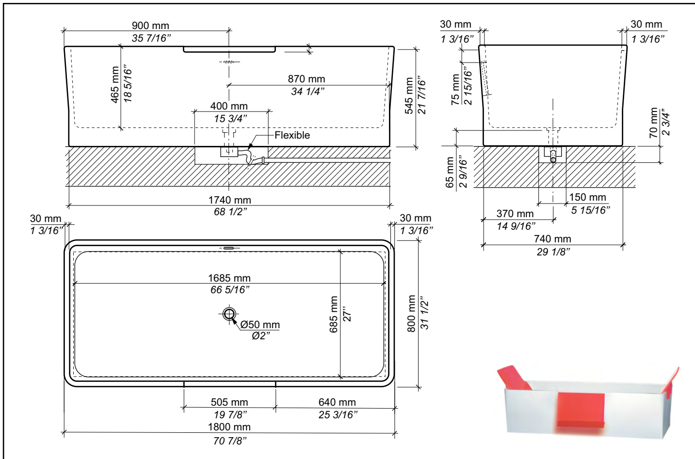
Dimensions en mm / in - Measurement in mm / in - Maatvoering in mm / in - Abmessungen in mm / in
