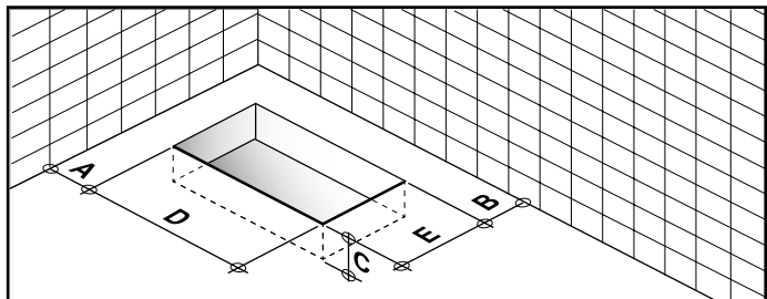
A = 500 mm / 19 11/16" - B = 175 mm / 6 7/8" - C = 70 mm / 2 3/4" - D = 400 mm / 15 3/4" - E = 150 mm / 5 15/16"
