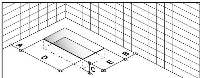
A = 550 mm / 30 1/2" - B = 275 mm / 9 13/16" - C = 120 mm / 4 3/4" - D = 400 mm / 15 3/4" - E = 250 mm / 9 13/16"
