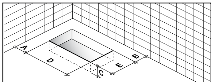
A = 700 mm / 26 3/4" - B = 375 mm / 13 3/4" - C = 70 mm / 2 3/4" - D = 400 mm / 15 3/4" - E = 150 mm / 5 15/16"
