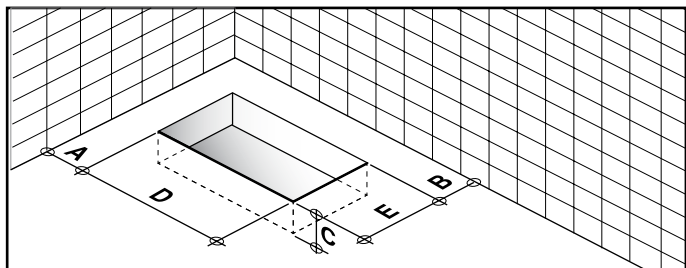
A = 700 mm / 26 3/4" - B = 375 mm / 13 3/4" - C = 120 mm / 4 3/4" - D = 400 mm / 15 3/4" - E = 150 mm / 5 15/16"
